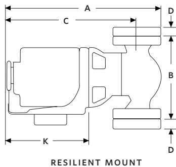
RESILIENT MOUNT
